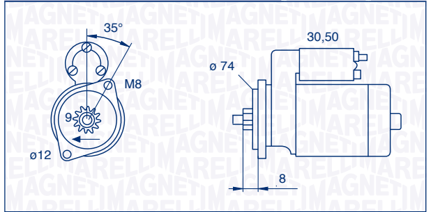
063280058010 – MSN8058 2,0 kW 12 V
