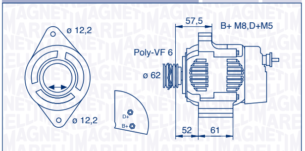
063377552010 – MAN7552 140 A 12 V
