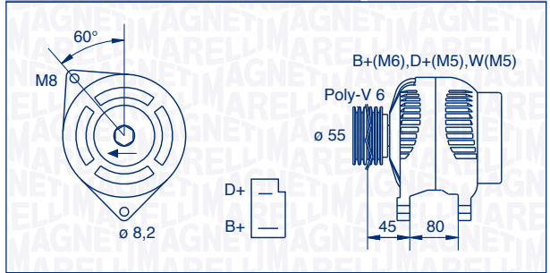
063321042010 – MAN283 55 A 12 V
