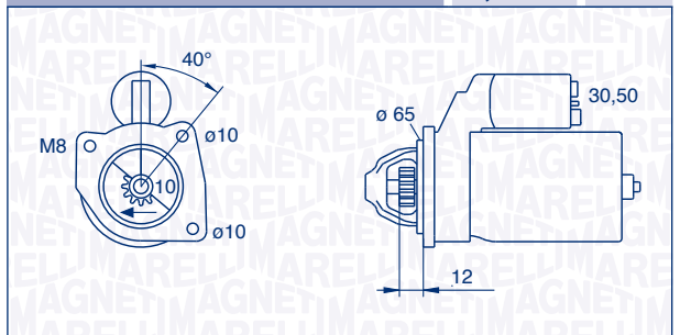
063280061010 – MSN8061 1,0 kW 12 V
