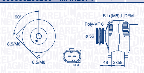
063535255250 – MAN2074 140 A 12 V
