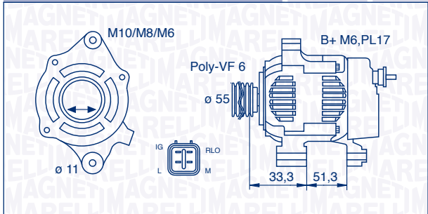
063377585010 – MAN7585 100 A 12 V
