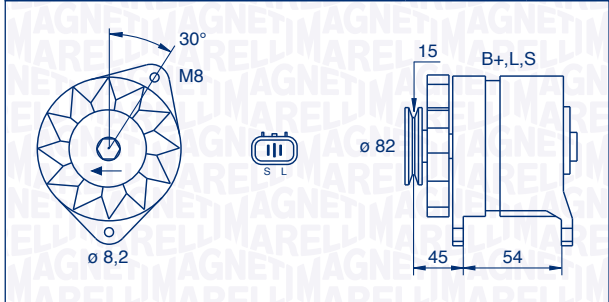
063532605010 – MAN2605 65 A 12 V
