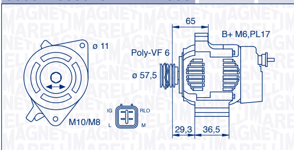
063377535010 – MAN7535 100 A 12 V
