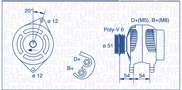
063321836010 – MAN1121 90 A 12 V
