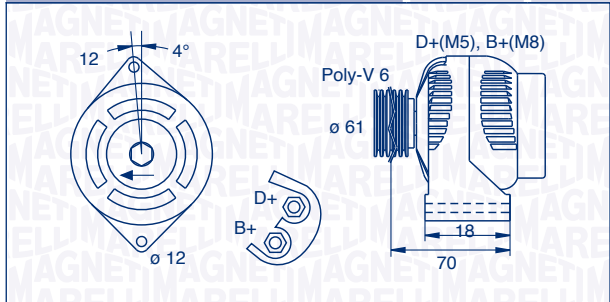
063377005010 – MAN7005 140 A 12 V
