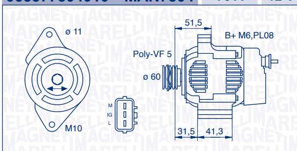
063377504010 – MAN7504 70 A 12 V
