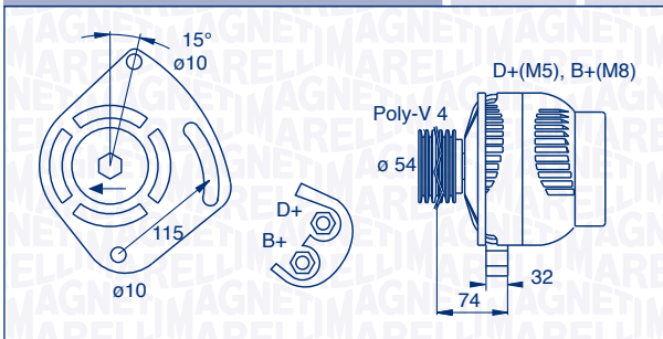
063377011010 – MAN7011 70 A 12 V
