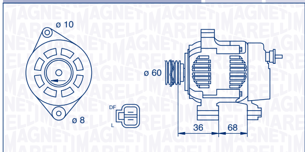
063533488010 – MAN2810 140 A 12 V
