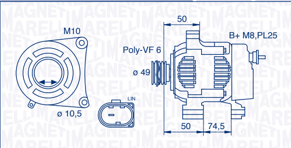
063377580010 – MAN7580 210 A 12 V
