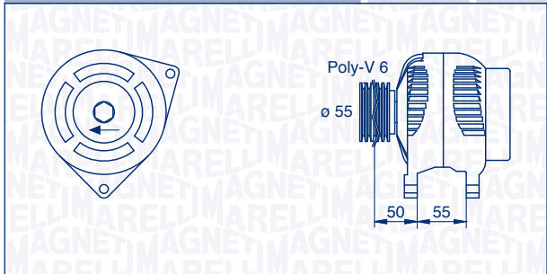
063377429010 – MAN7429 70 A 12 V
