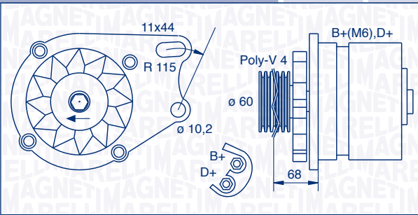
063321761010 – MAN1150 75 A 12 V
