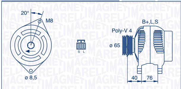
063532623010 – MAN2623 90 A 12 V
