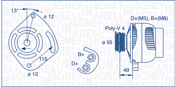
063321715010 – MAN1039 90 A 12 V
