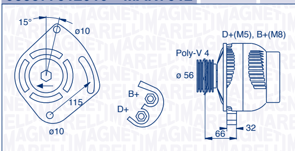
063377012010 – MAN7012 70 A 12 V
