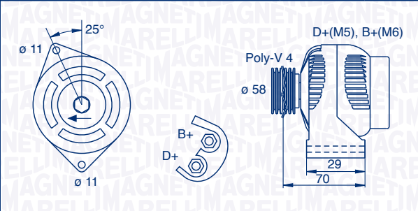
063341702010 – MAN1008 65 A 12 V
