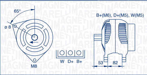
063377462010 – MAN7462 85 A 12 V
