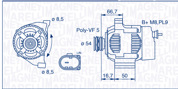
063377561010 – MAN7561 120 A 12 V
