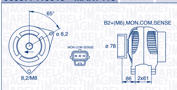
063377413010 – MAN7413 90 A 12 V
