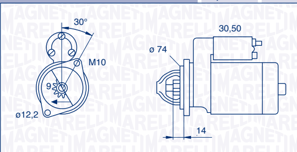
063280055010 – MSN8055 1,0 kW 12 V
