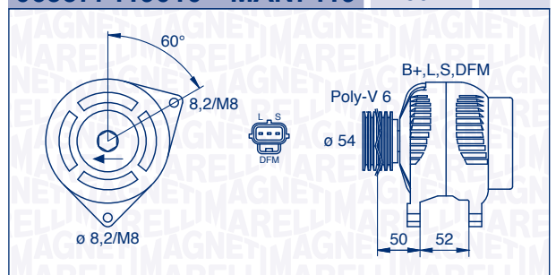
063377419010 – MAN7419 150 A 12 V
