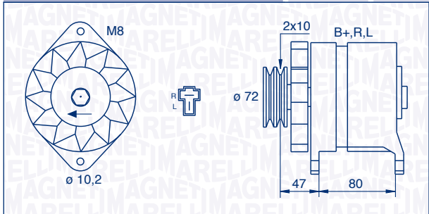
063532621010 – MAN2621 60 A 12 V
