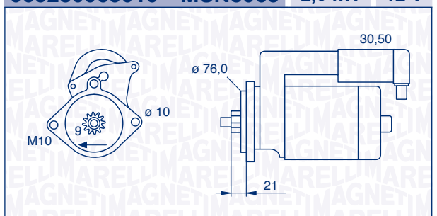
063280063010 – MSN8063 2,0 kW 12 V
