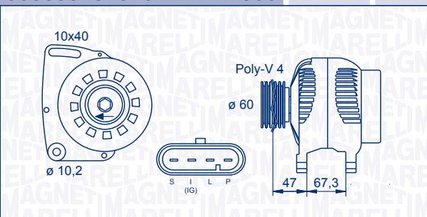
063533484010 – MAN2806 75 A 12 V
