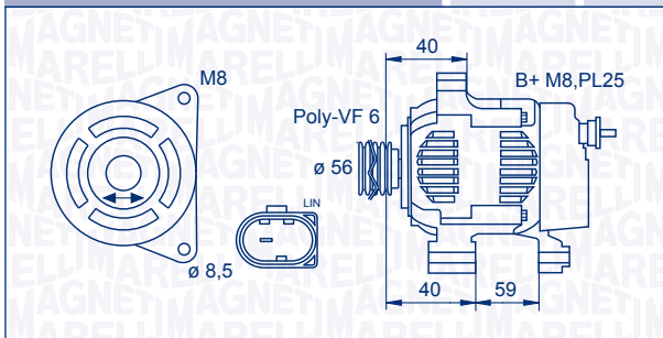
063377588010 – MAN7588 140 A 12 V
