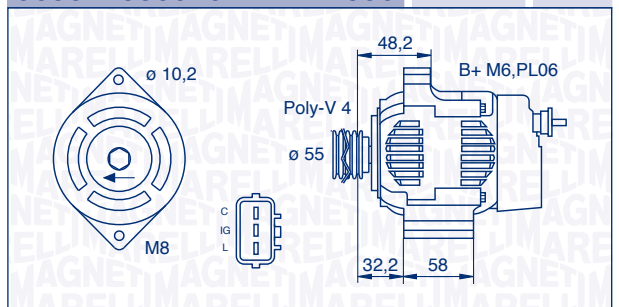
063377530010 – MAN7530 75 A 12 V
