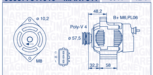
063377511010 – MAN7511 50 A 12 V
