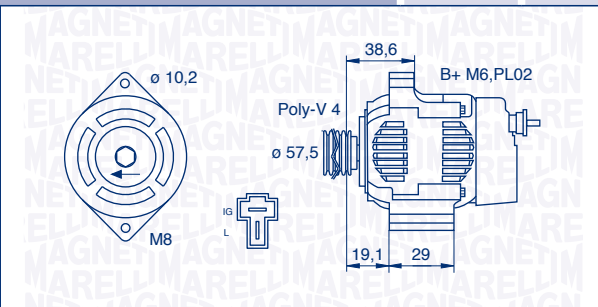
063377513010 – MAN7513 60 A 12 V
