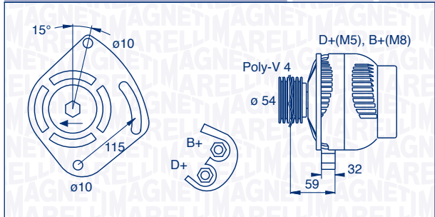
063377001010 – MAN7001 70 A 12 V
