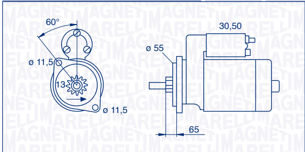
063280050010 – MSN8050 1,2 kW 12 V
