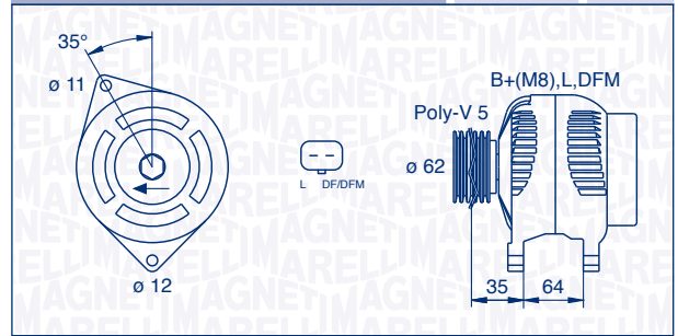
063377015010 – MAN7015 150 A 12 V
