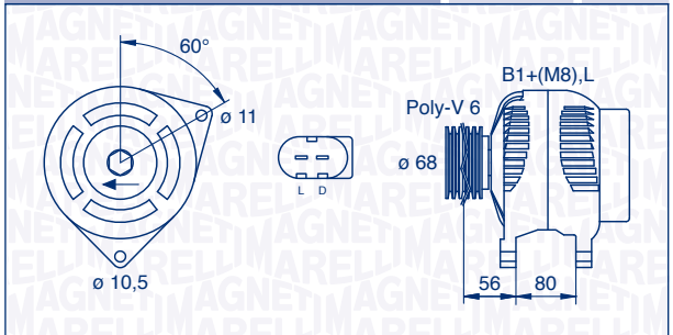
063535150440 – MAN2030 120 A 12 V
