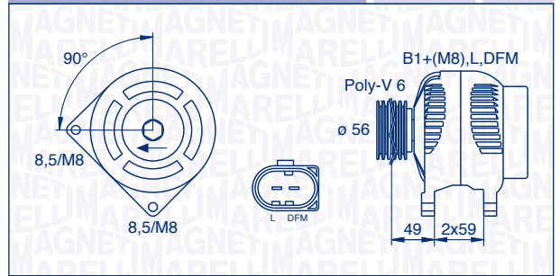
063533250010 – MAN2037 90 A 12 V
