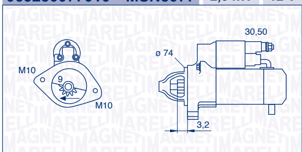
063280077010 – MSN8077 2,0 kW 12 V
