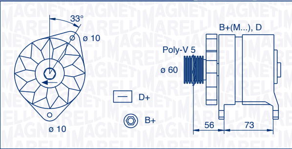
063321155010 – MAN320 55 A 12 V
