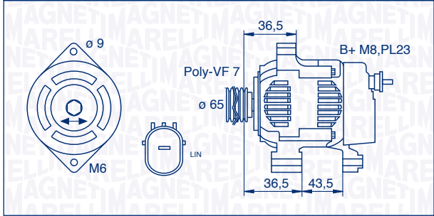
063377582010 – MAN7582 150 A 12 V
