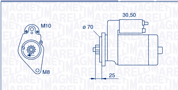
063280089010 – MSN8089 2,0 kW 12 V
