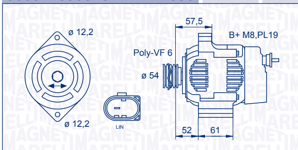
063377590010 – MAN7590 120 A 12 V
