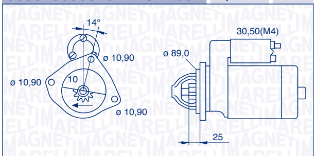
063523680820 – MSN2057 4,0 kW 24 V
