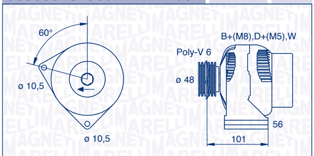
063535151900 – MAN2087 120 A 12 V
